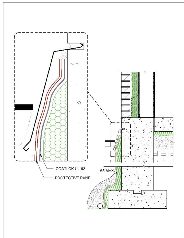
Figure 2 Coatlok U-192 membrane applied on SPF Heatlok Soya
