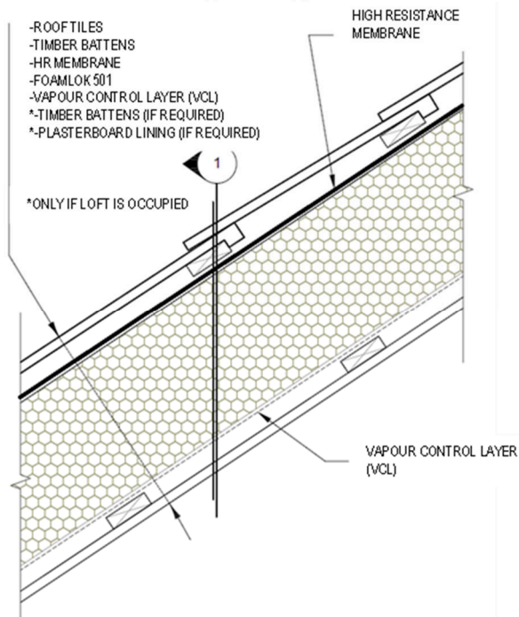
Diagram 2 - Elevation detail of typical loft application with HR membrane
