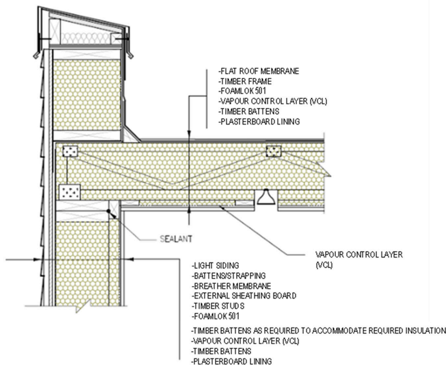
Diagram 1 - Elevation detail of typical timber-frame flat roof
