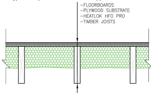
Diagram 1 - typical suspended timber floor - application from below detail
