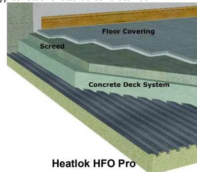
Diagram 4 - typical steel-shuttered concrete floor
