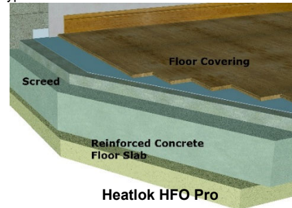
Diagram 2 - typical concrete floor detail
