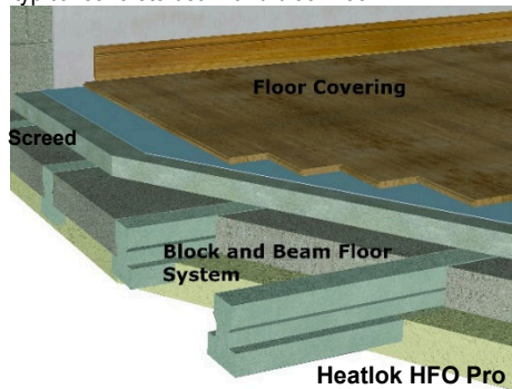
Diagram 3 - typical concrete beam and block floor
